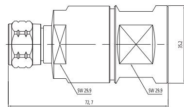
N-Male for 7/8"
