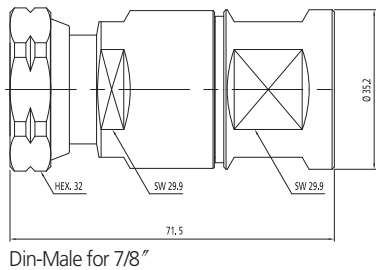
Din-Male for 7/8"
