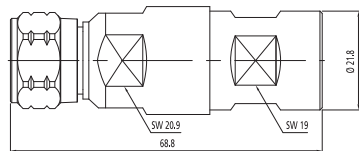
N-Male for 1/2"
