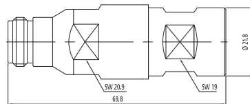
N-Female for 1/2"
