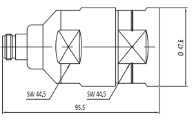
N-Female for 1-1/4"
