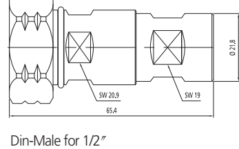
Din-Male for 1/2"
