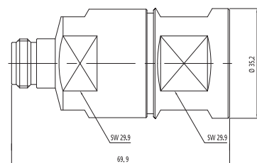
N-Female for 7/8"
