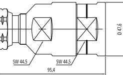
Din-Male for 1-1/4"
