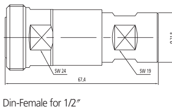
Din-Female for 1/2"
