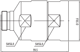
Din-Female for 1-5/8"
