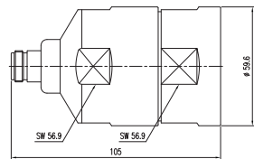
N-Female for 1-5/8"
