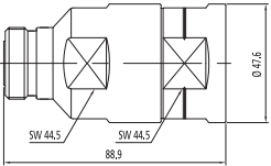
Din-Female for 1-1/4"
