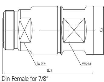
Din-Female for 7/8"
