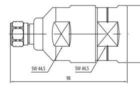
N-Male for 1-1/4"
