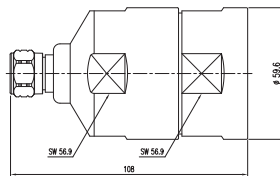
N-Male for 1-5/8"
