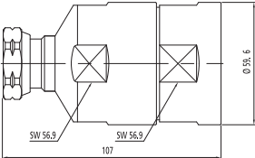
Din-Male for 1-5/8"
